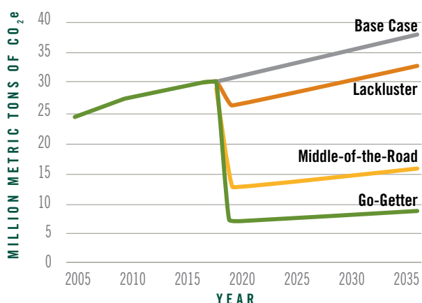
FIGURE A-1.17 Nitrous Oxide Emissions from Nitric and Adipic Acid Manufacturing
